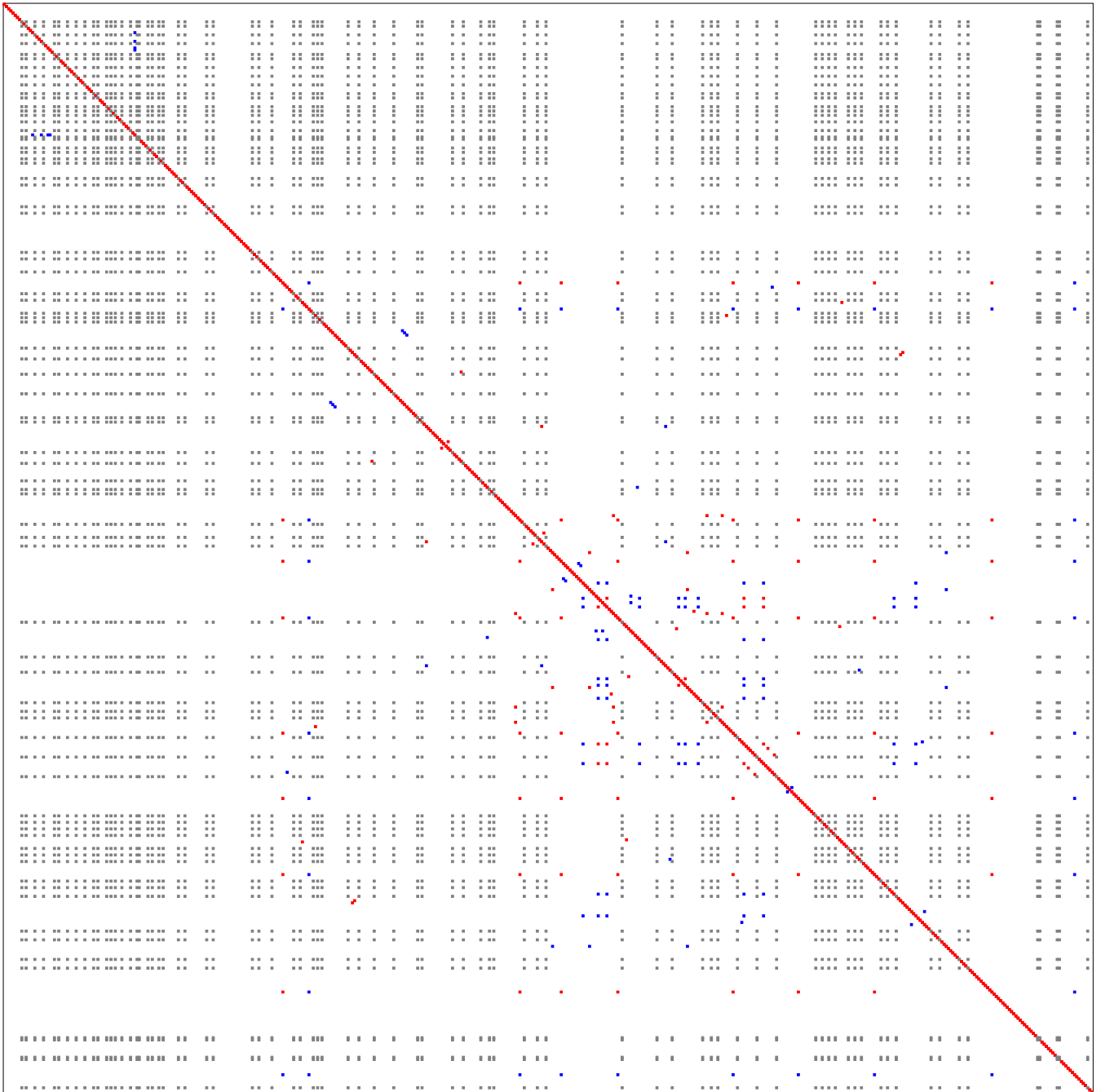
EditorWindow.py
